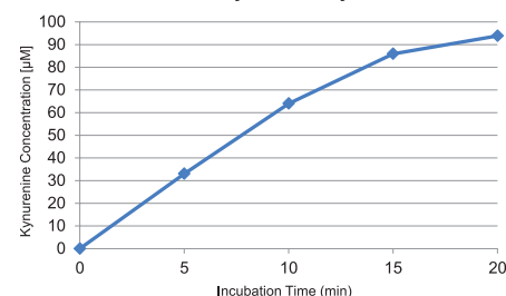
IDO1 Enzymatic Assay
